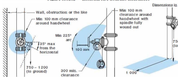
Figure H.3(B) — Internal fire hydrant clearances
