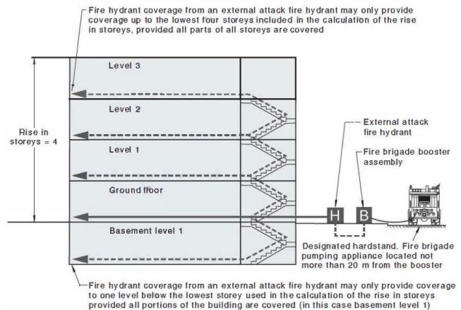
Figure H.6.1.3 — External attack fire hydrant coverage
