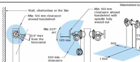
Figure H.3(A) — External fire hydrant clearances
