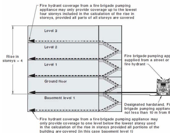
Figure H.6.1.2(A) — Coverage from a fire brigade pumping appliance
